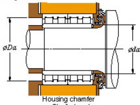
53FC37234B Bearing 2D drawings and 3D CAD models
